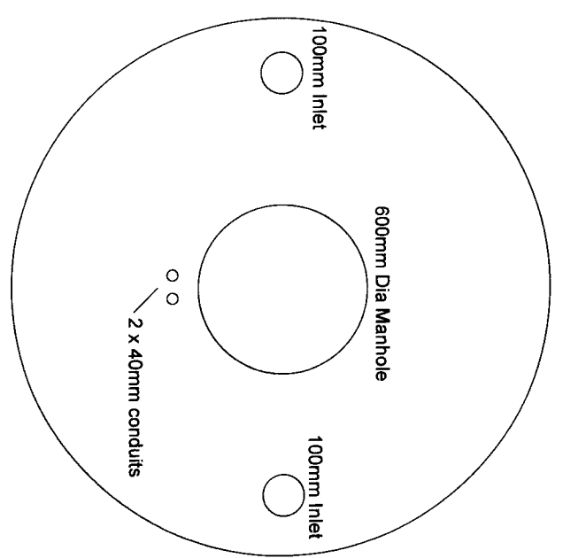
Plan View of Lid
